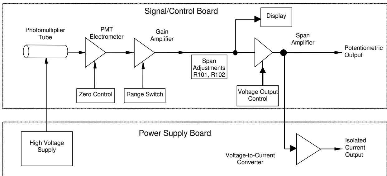
Figure 4-1. Analyzer Block Diagram
